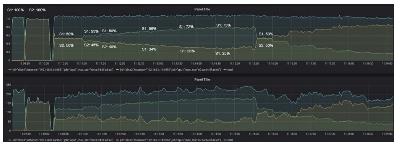
Figure 3-3. Evaluating airtime scheduling with 802.11n/ath9k 40MHz channel – airtime per slice (upper) and throughput per slice (lower).
