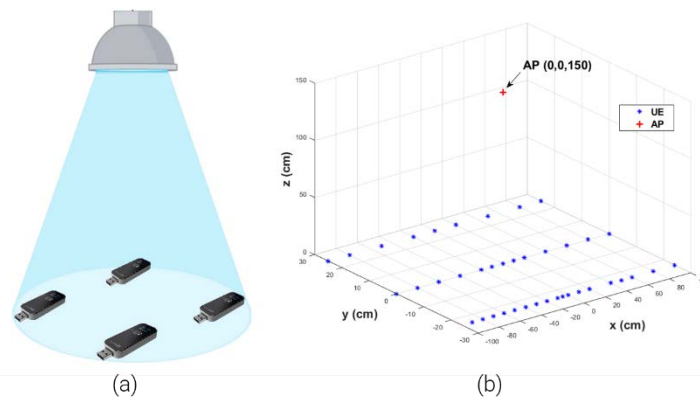
Figure 4-12: RSSI measurement using LiFi dongle (UE), (a) stationary measurement, (b) coordinates of AP and UE locations
