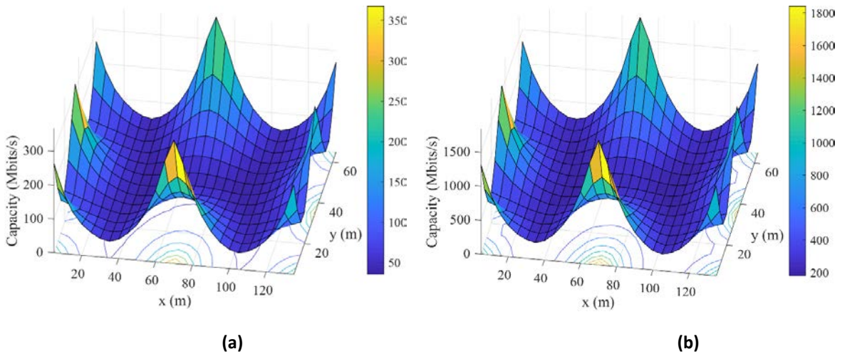
Figure 5-16. The capacity for 5GNR-I (3.5 GHz) APs in the dense scenario, (a) conservative, and (b) opportunistic approaches.
