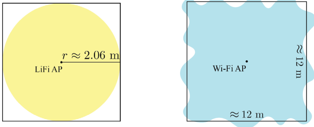
Figure 5-5 Coverage area assumptions for LiFi (left) and Wi-Fi (right) APs.
