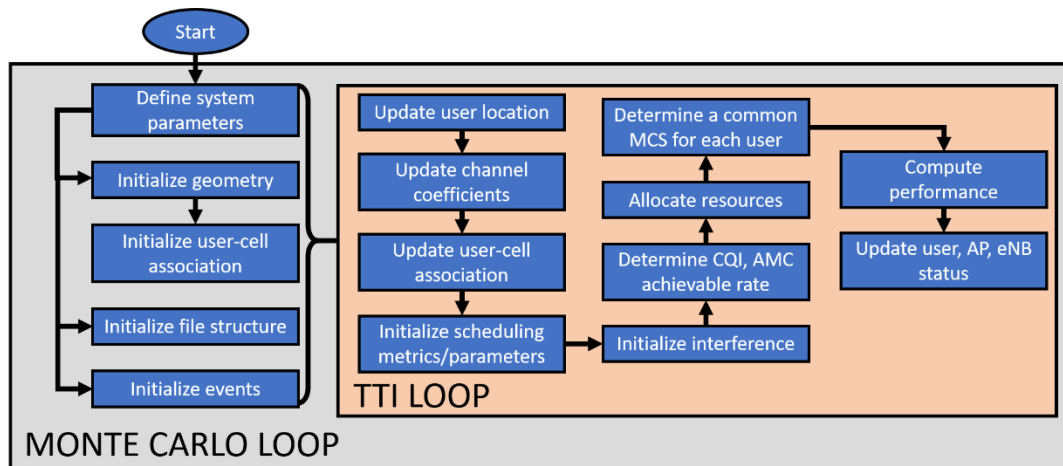
Figure 5-2: The building blocks for multi-WAT traffic simulator.
