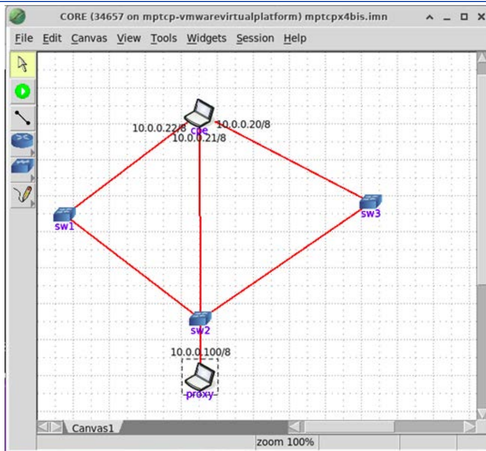
Figure 2-41: Experimental topology implemented in CORE-EMU environment, featuring a CPE with three network interfaces, and a MPTCP proxy with only one interface.
